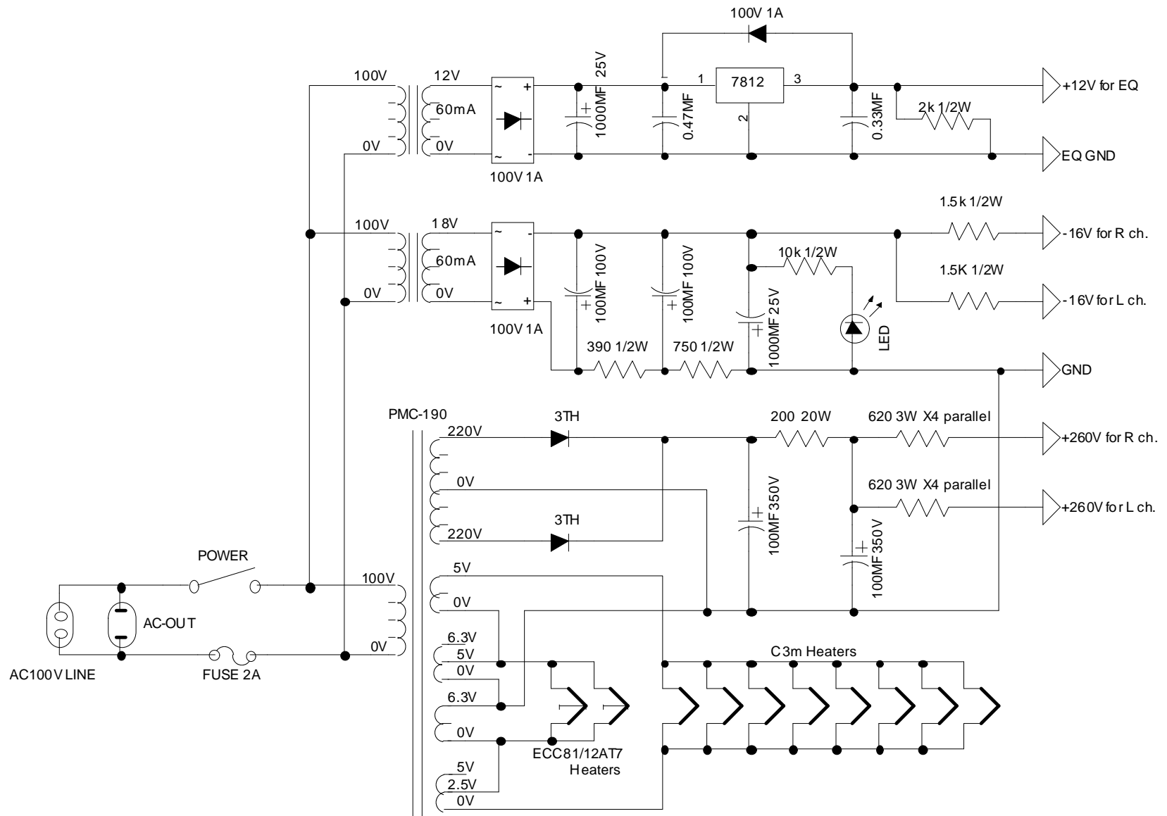
POWER SUPPLY
